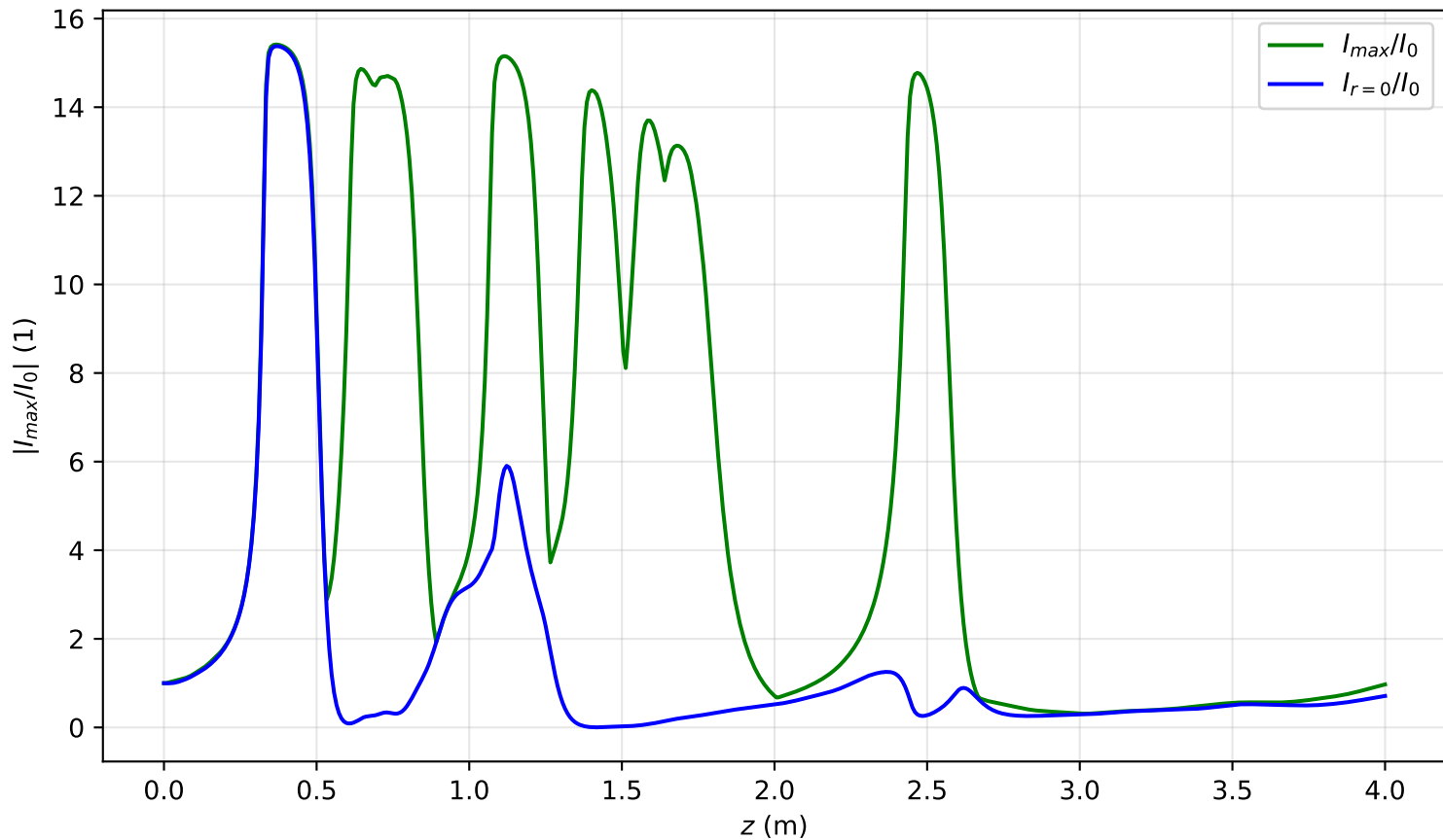
I_{max}(x=0, y=0, z)/I_0 , P_{in}=7.2P_{cr} , noisy input, artificial time
